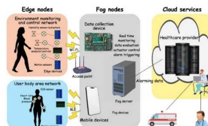
Fig. 2. Edge-to-Cloud Architecture Layers
